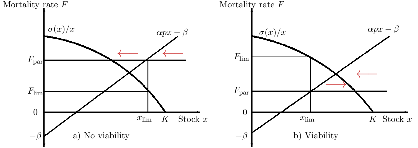
Figure 1: Two contrasted cases for viability: In case a) when F_{\text{lim}} < F_{\text{par}} , no viability occurs and the viability kernel \text{Viab} = \emptyset is empty. In case b) when F_{\text{lim}} \geq F_{\text{par}} , the viability kernel is \text{Viab} = [x_{\text{lim}}, \infty[ .
